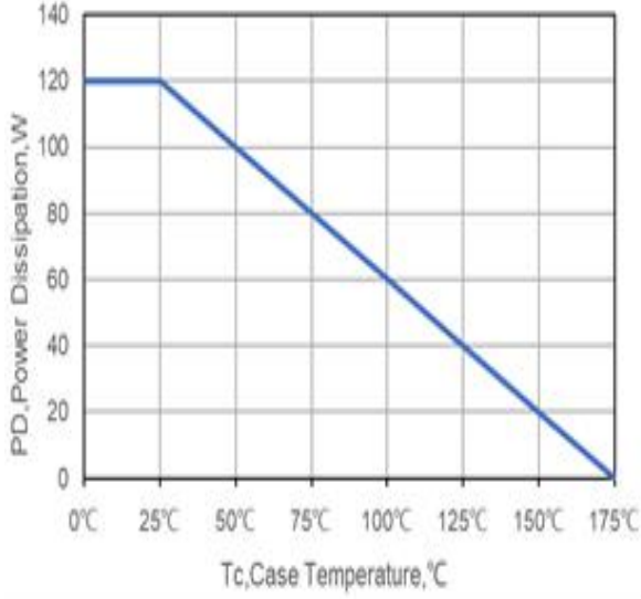
Figure 5. Power De-rating
